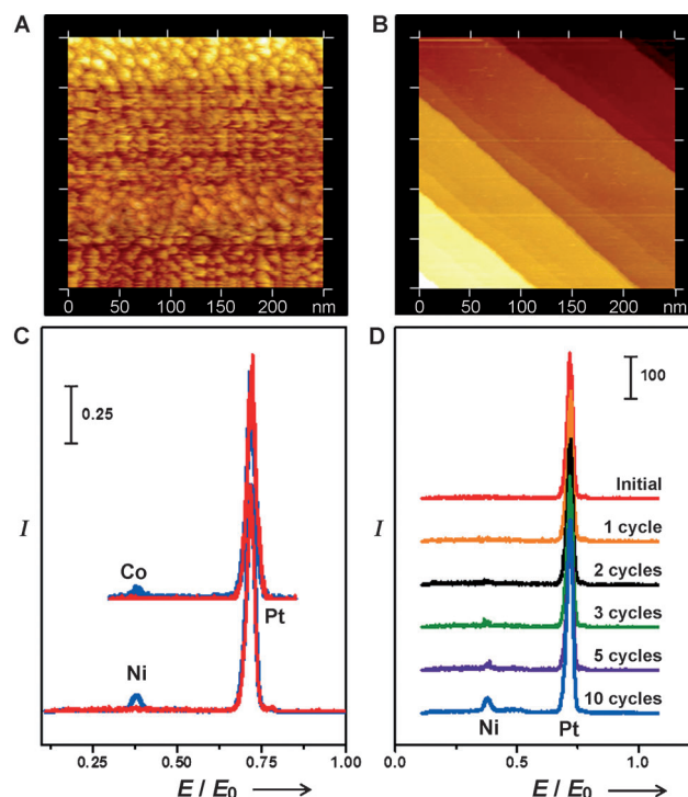
Figure 1. Surface characterization of Pt 3 M(111) surfaces in UHV: STM images of A) sputtered and B) annealed Pt 3 Ni(111) surfaces. The brightness in colors is a measure of the depth profile, with each color change marking a single atomic step. Low-energy ion scattering spectra of C) sputtered (blue traces) versus annealed (red traces) surfaces of Pt 3 Ni(111) and Pt 3 Co(111) crystals. D) Successive LEIS spectra of Pt 3 Ni(111) surface during Ne-sputtering. The graphs in (C) and (D) are shifted, and the scale bars indicate the intensities in arbitrary units. E/E_0 is the ratio of the energy of the scattered ion beam ( E ) and the energy of the incident ion beam ( E_0 ).
